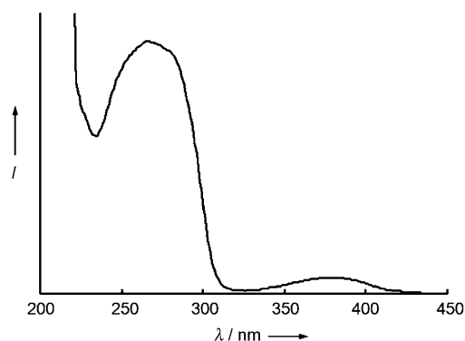
Figure 4. Excitation spectrum of coumarin 1/biphenyl-PMO film (1.2 mol %, C_{18}TMACl , (400 \pm 50) nm thickness). The emission was detected at 440 nm.
