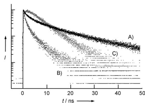
Figure 5. Fluorescence decay profiles of biphenyl-PMO powder monitored at 370 nm (A), and coumarin 1/biphenyl-PMO powder (0.66 mol %) monitored at 370 nm (B), and 500 nm (C) (excitation wavelength, 266 nm). The solid line for biphenyl-PMO is fitted by convolution of the instrument response function and quadruple-exponential function.
